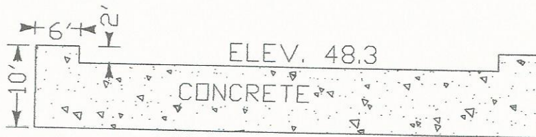
WEIR WALL FRONT LOOKING D/S
