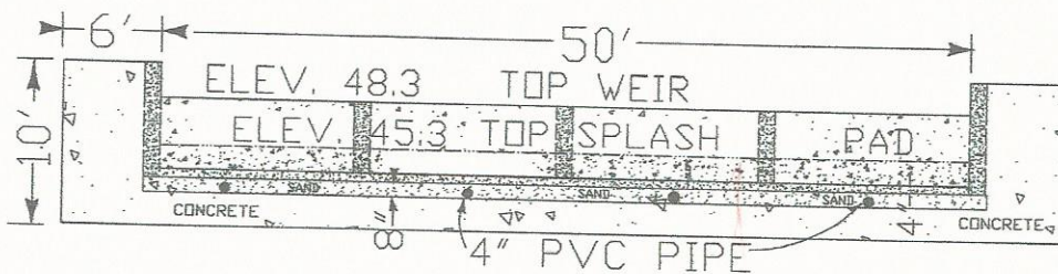
LOOKING U/S 62'
