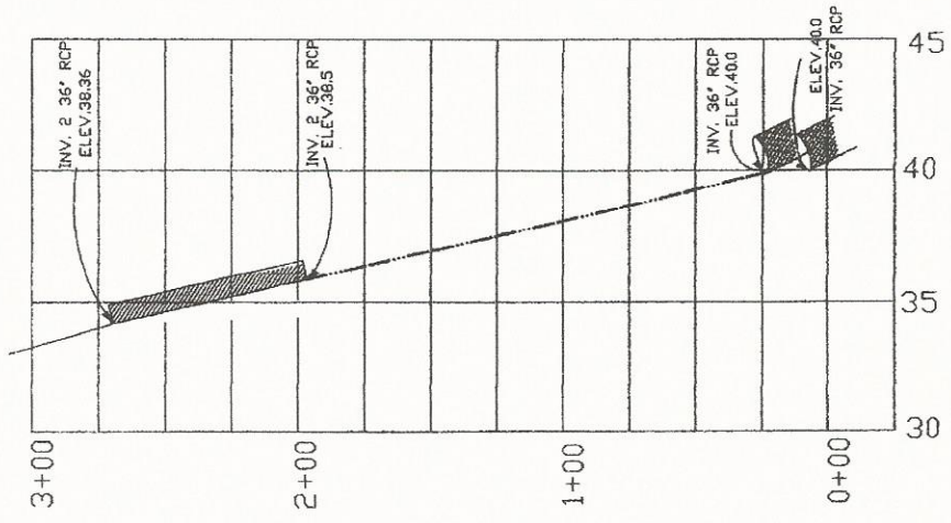
PROFILE C/L DITCH
